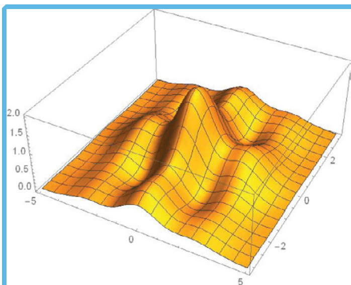
Figure 4: Maximum increase in temperature for core-shell Californium nanospheres with various thicknesses of silica shell.
