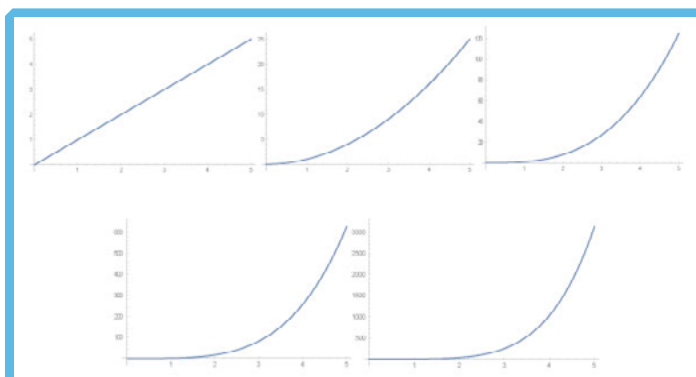
Figure 6: Extinction cross section area for Californium nanorods with effective radius of 45 (nm) and various dimension ratios.
