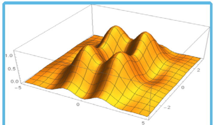
Figure 1: Maximum increase in temperature for Californium nanospheres.
